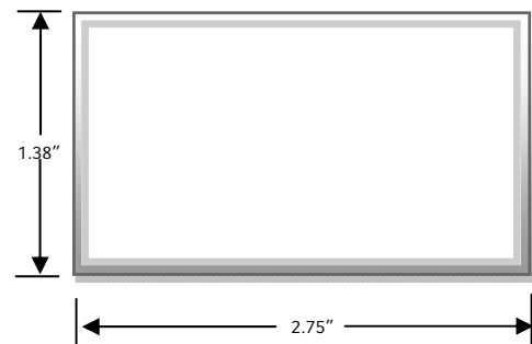
ECA Telecom Plate Cutout Dimensions
